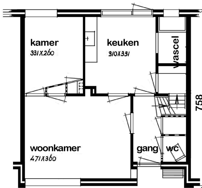
BEGANE GROND TYPE C
