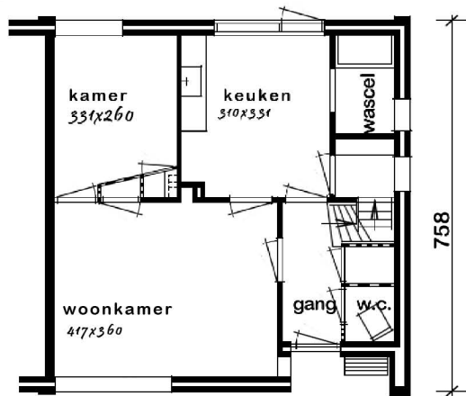
BEGANE GROND TYPE C 2
