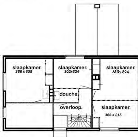
VERDIEPING.
